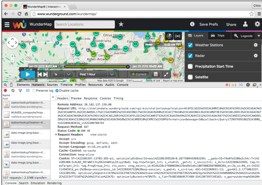
Figure 16-5: Viewing additional information about a particular record in the Network tab.
