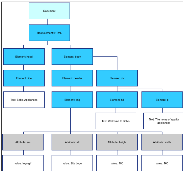
Figure 10-1: A representation of the Document Object Model for Listing 10-1.
